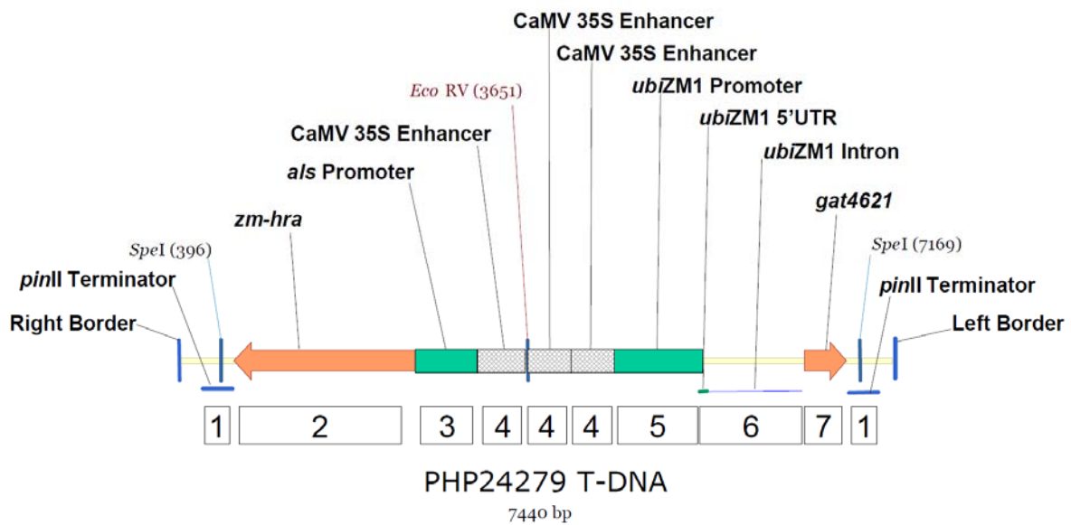
Figure 5. Map of PHP24279 T-DNA with genetic element probes indicated. Base pair positions for EcoRV and SpeI restriction enzyme sites are also shown. The total T-DNA size is 7440 base pairs. Probes used for Southern blotting are indicated schematically as numbered boxes below the map. Probe 1: pinII terminator; 2: zm-hra ; 3: als promoter; 4: 35S enhancer; 5: ubiZM1 promoter; 6: ubiZM1 intron; 7: gat4621 .
